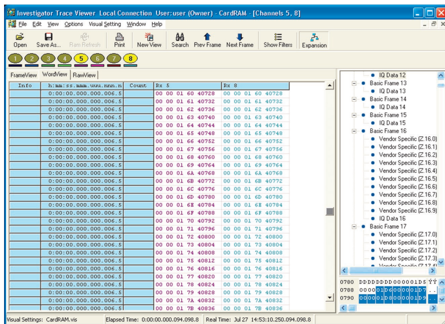
Investigator Trace Viewer showing a CPRI word view trace
